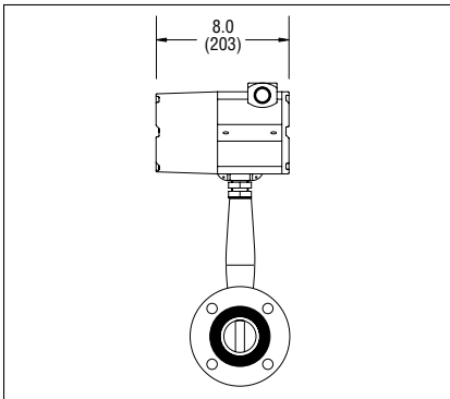
240 Wafer—Side View
