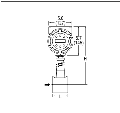
240 Wafer—Outlet View
