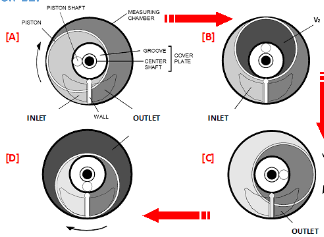
Figure 1 Measurement Principle
